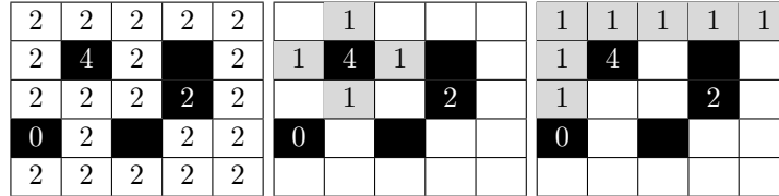
■ Figure 2 Illustrations for steps 1 to 3 in the Akari ZKP construction. From left to right: Step 1: two cards added on all white cells. Step 2: cards added around black cells with number. Step 3: cards added per cell as a function of adjacent cells.
